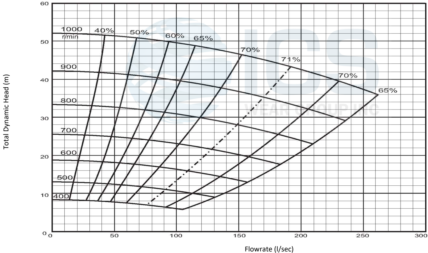
Curve Ref: ICSDPF86RRCLP
